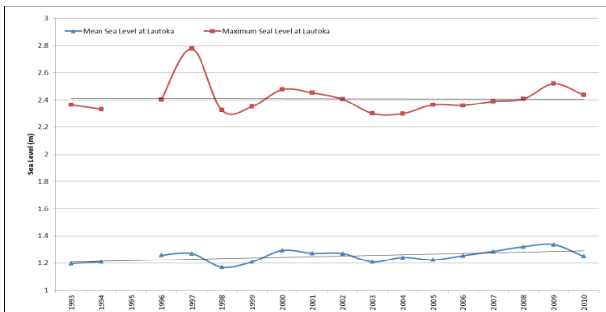
Figure A1-5: Trends in mean and maximum sea levels at Lautoka tide gauge, 1993–2010 Data source: South Pacific Sea Level and Climate Monitoring Project.
