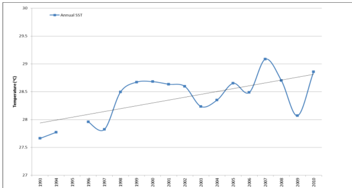
Figure A1-4: Annual sea surface temperature trends at the Lautoka tide gauge, 1993–2010 Data source: South Pacific Sea Level and Climate Monitoring Project.
