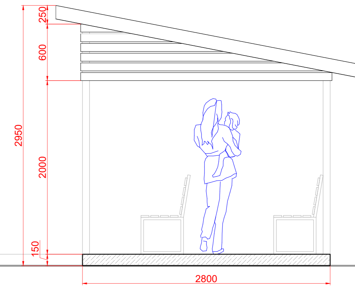
Side elevation
