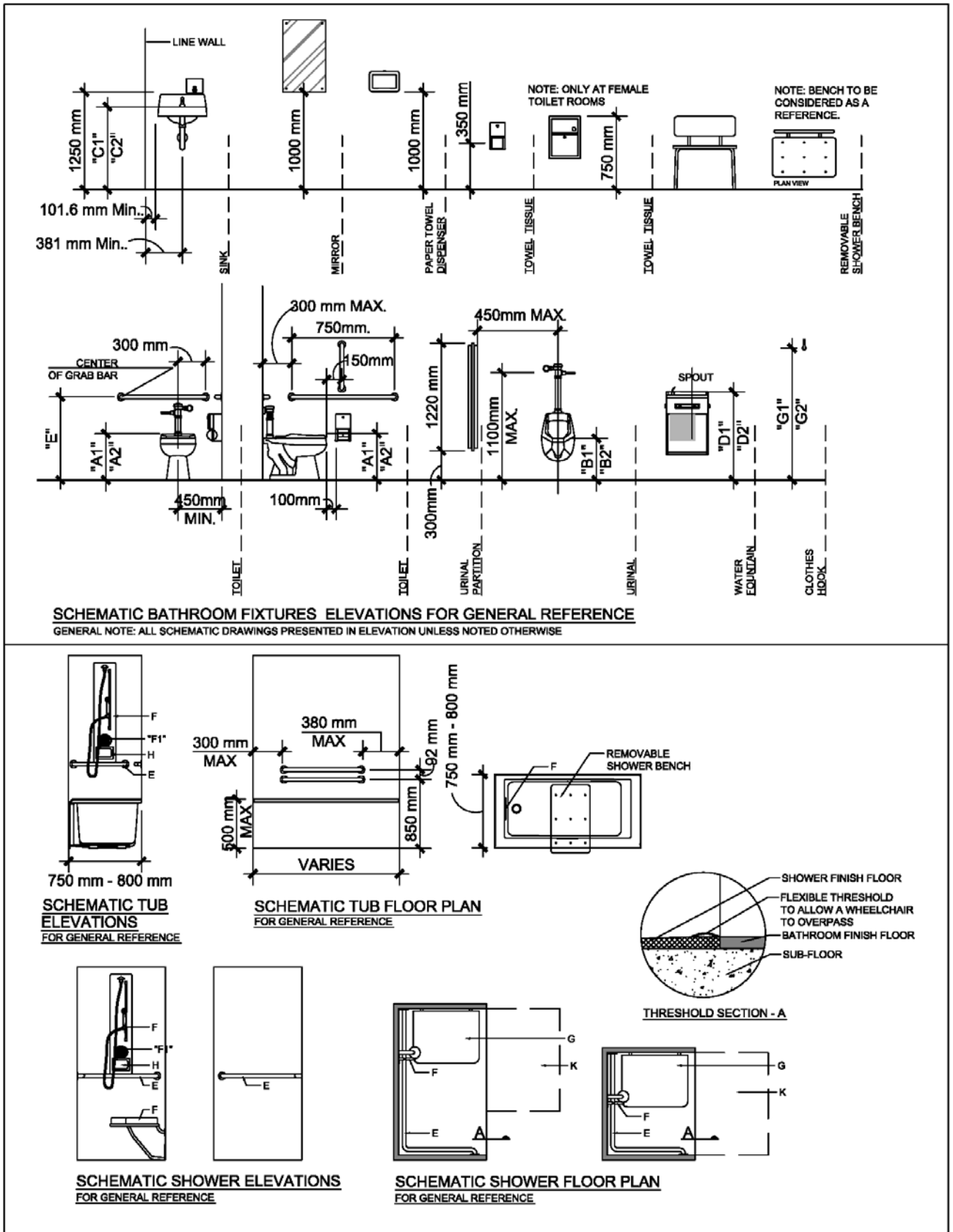
Figure 42: Bathroom fixtures schematic
