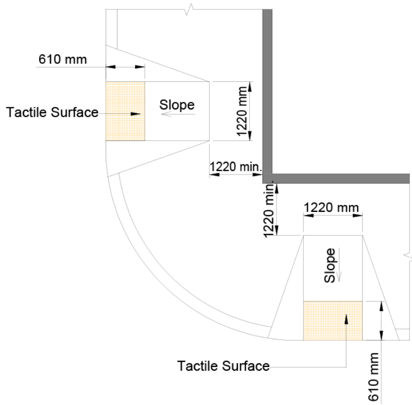
Figure 22: Kerb ramp at corner
