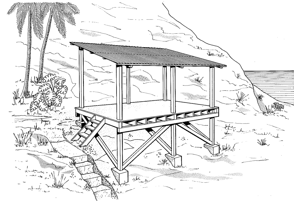
Figure 7 BRE-HLDC St Vincent low-income house (type 2) — 19 square metres
