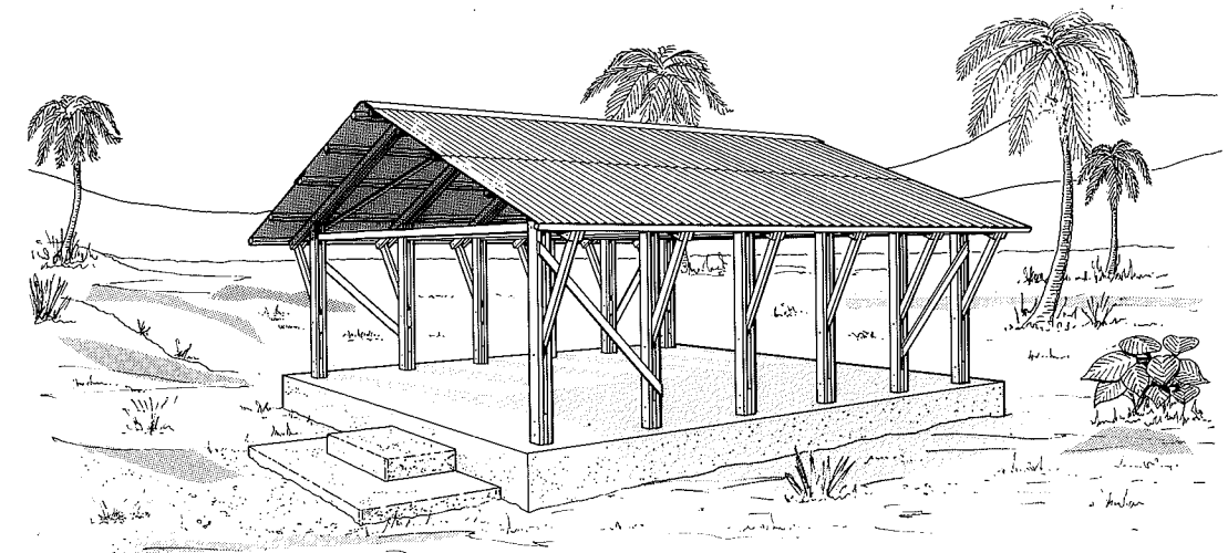
Figure 8 BRE-HLDC St Vincent low-income house/community building — 51 square metres
