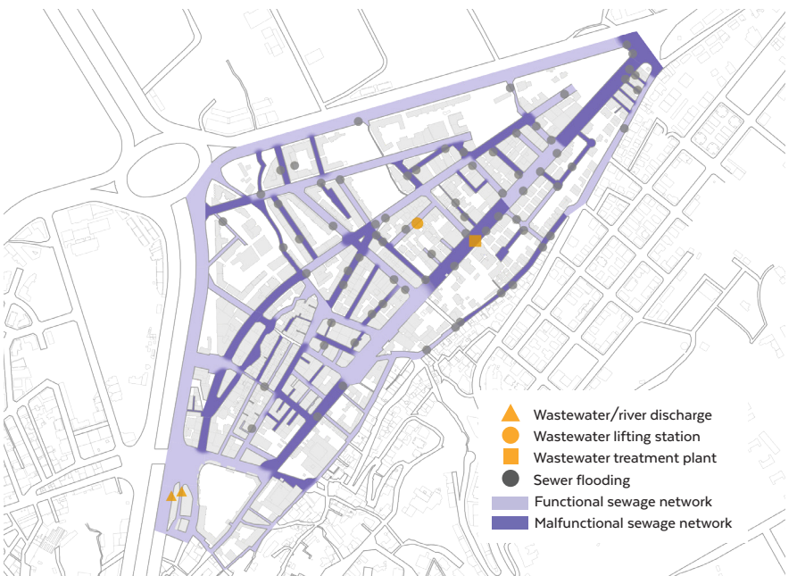
Figure 46 Street mapping of wastewater network
