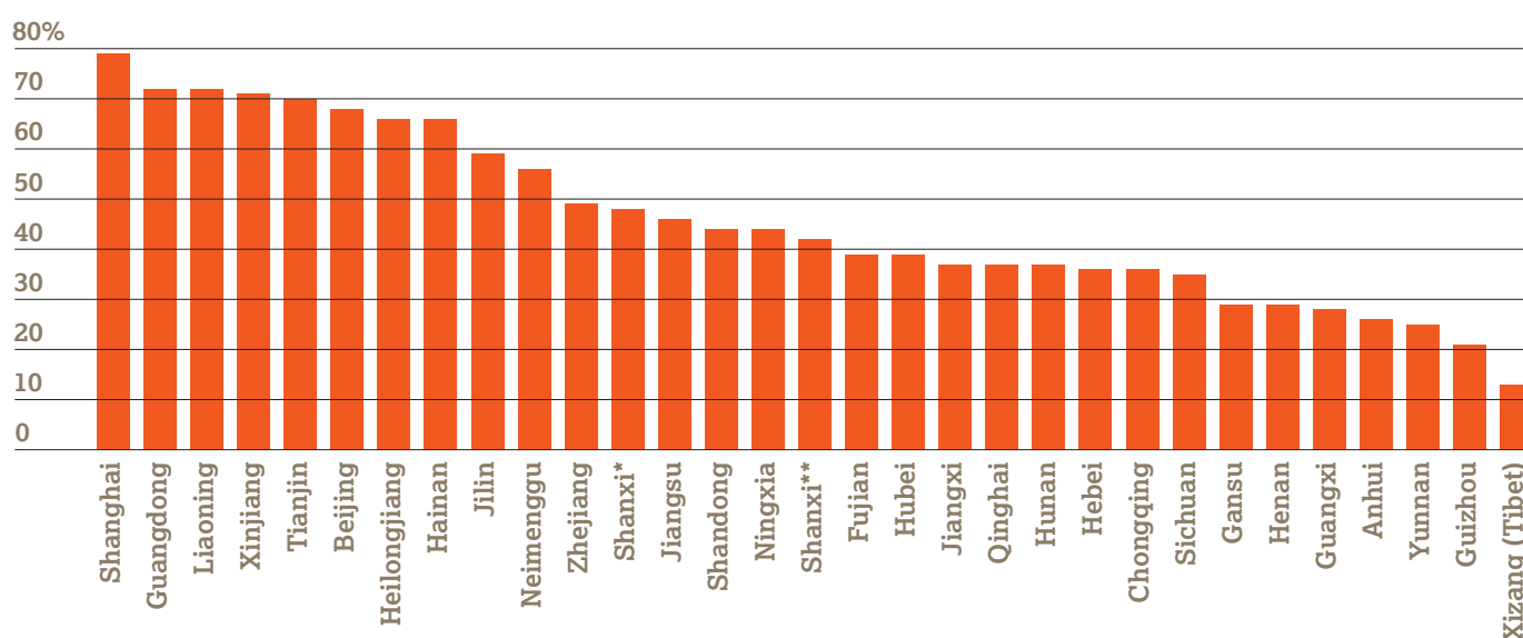
Figure 3: Coverage rates of BOISE in 31 provinces in China (2010)
