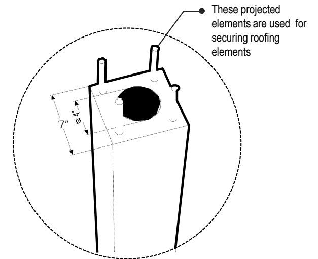
2 Blow up of Column Head
