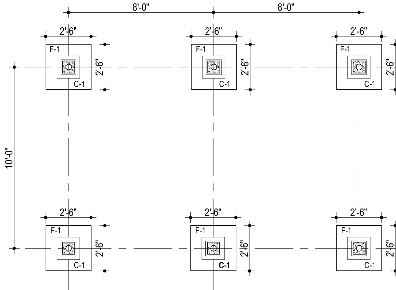
Footings and Column Layout Plan
