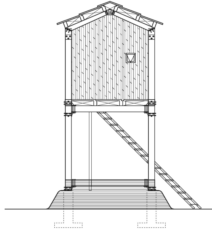
Side Elevation
