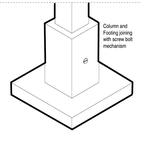
② RCC/FC Column joint with stump pad footing using screw joint
