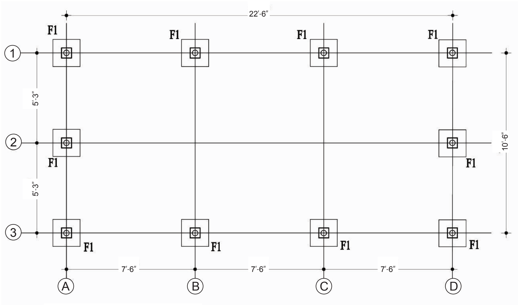
Foundation layout
