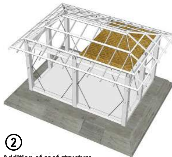
Addition of roof structure
