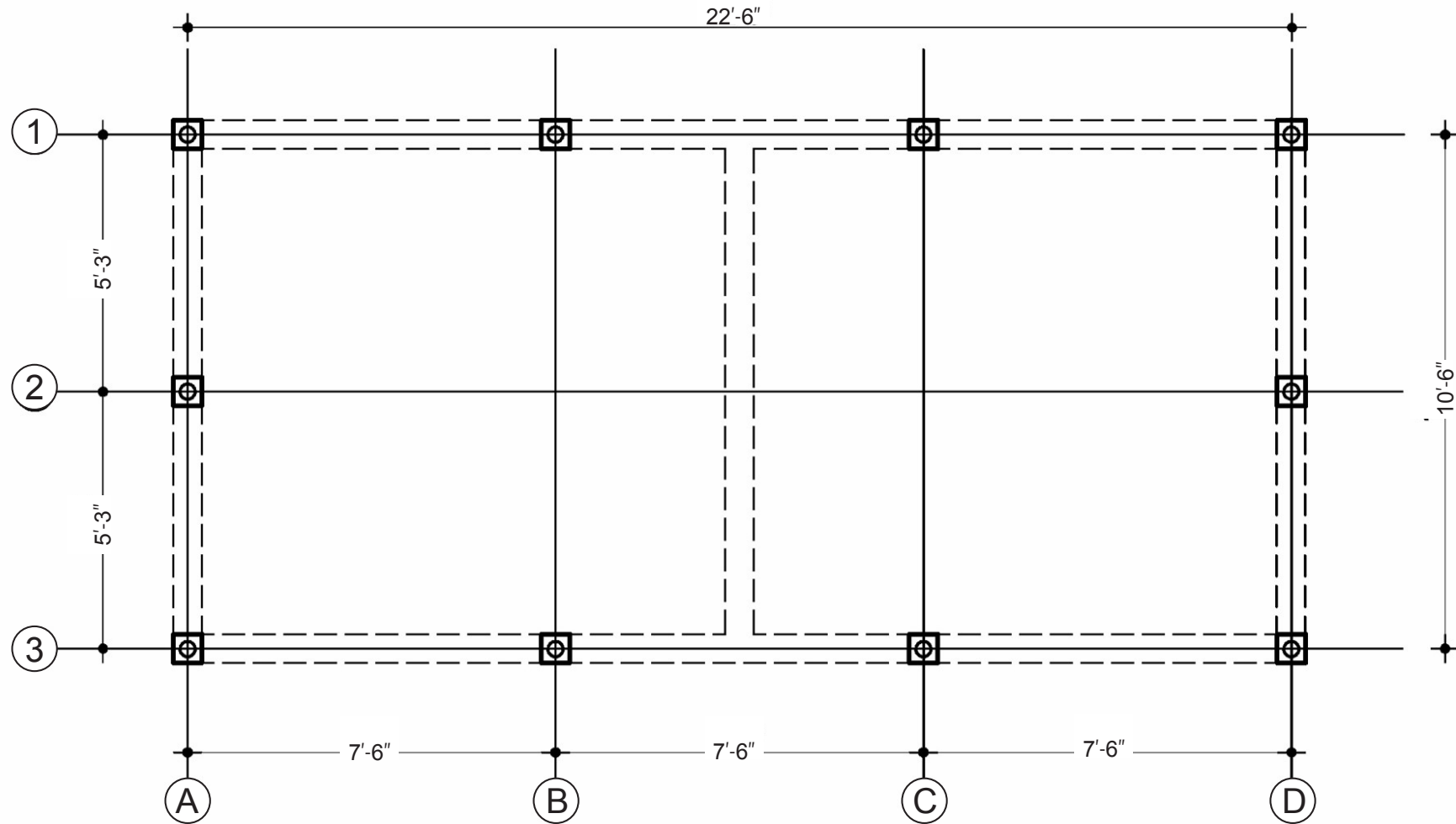
Beam-Column layout
