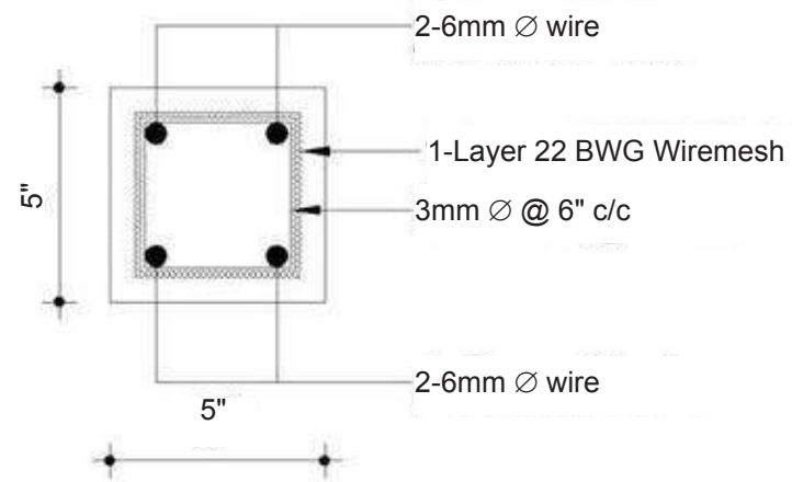
Section of Lintel
