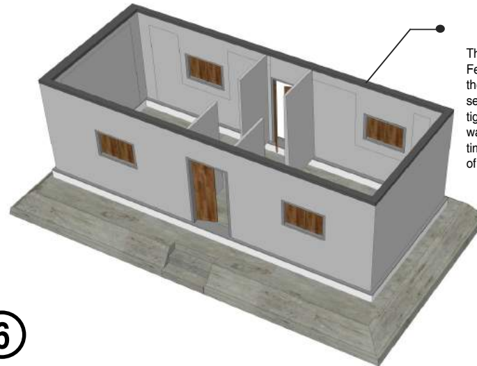
Superstructure with Ferrocement Band
