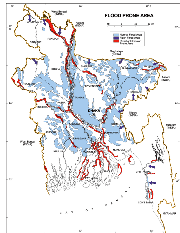
Map of three types of flooding: regular flooding, flash flooding and river erosion
