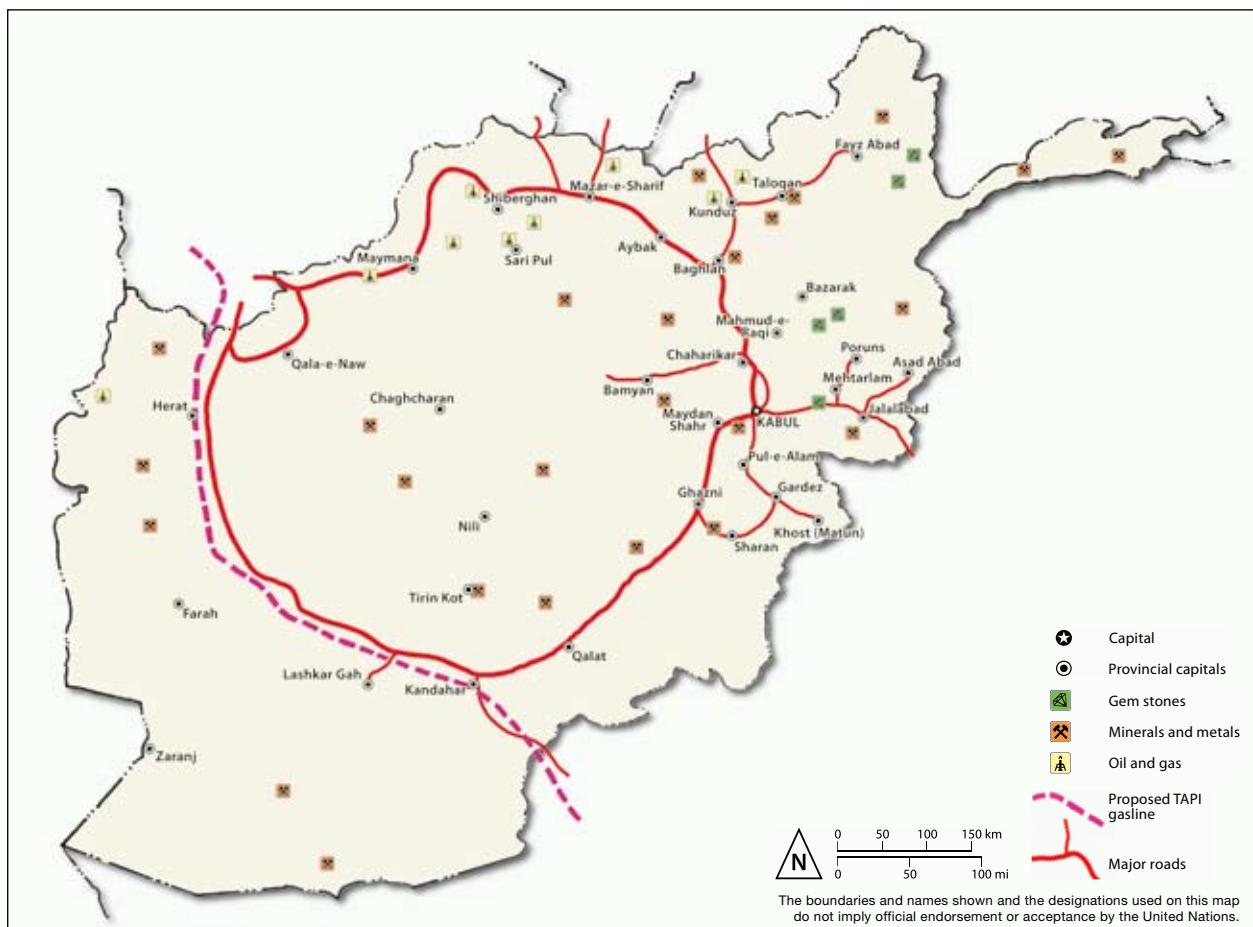
Map 6. Mineral availability in Afghanistan
