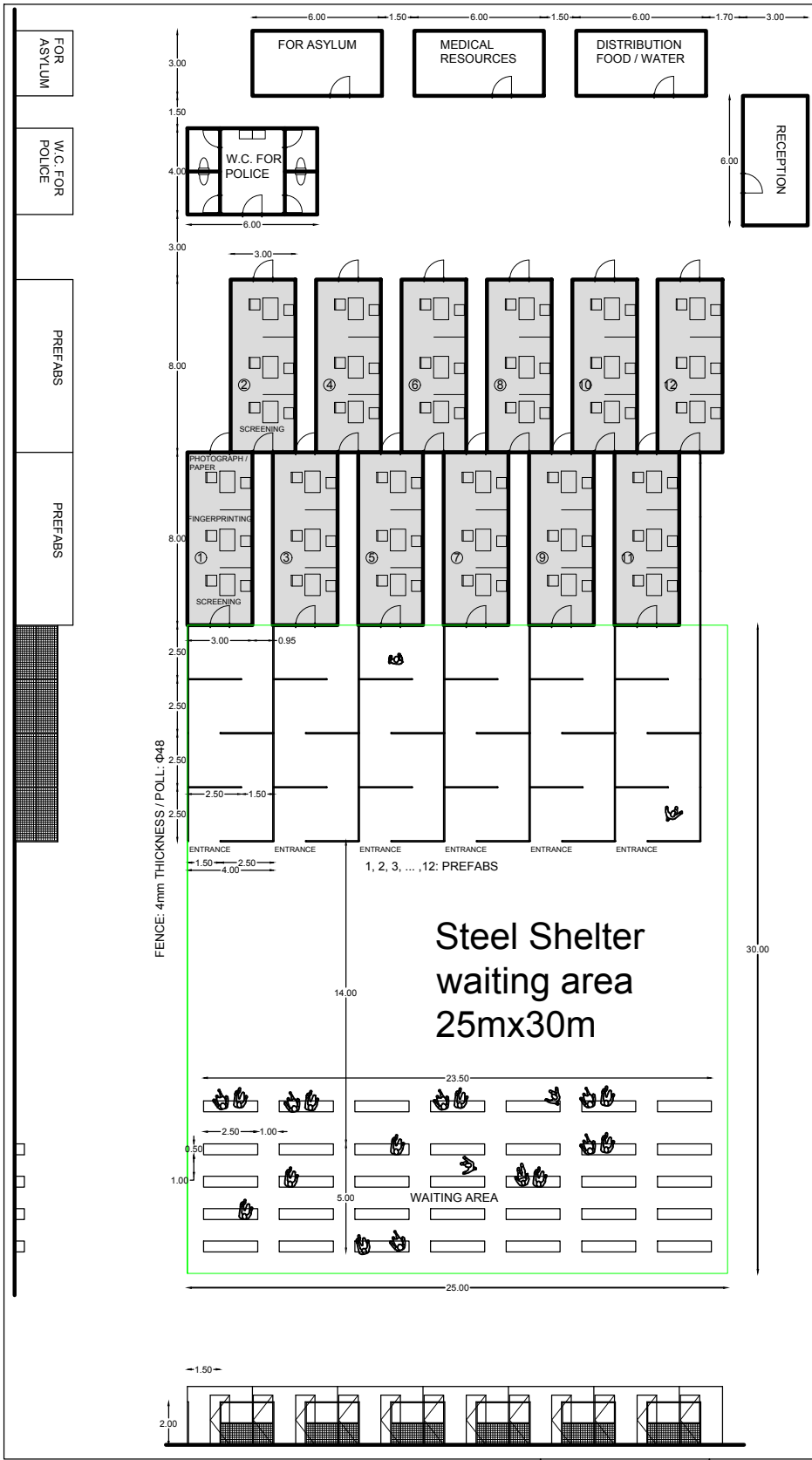
Plan for Registration in Moria Drawing No 6
